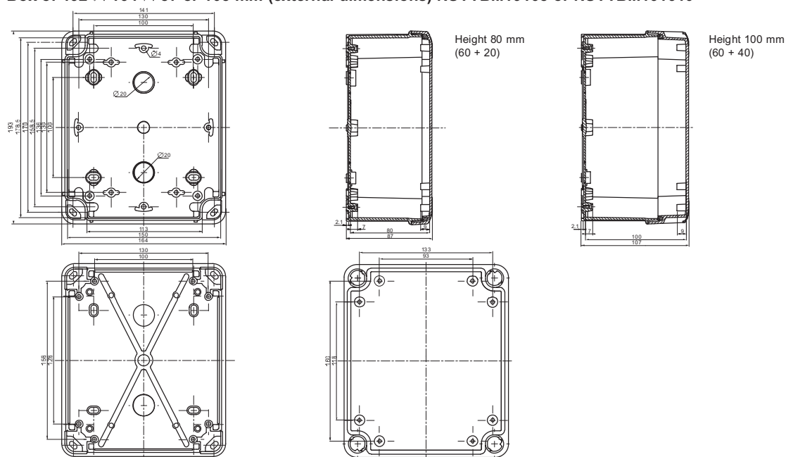
Box of 192 × 164 × 87 or 105 mm (external dimensions) NSYTB...19168 or NSYTB...191610
