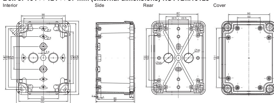
Box of 192 × 121 × 87 or 105 mm (external dimensions) NSYTB...19128 or NSYTB...191210
