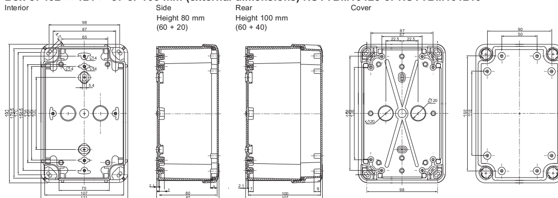
Box of 192 × 164 × 87 or 105 mm (external dimensions) NSYTB...19168 or NSYTB...191610
